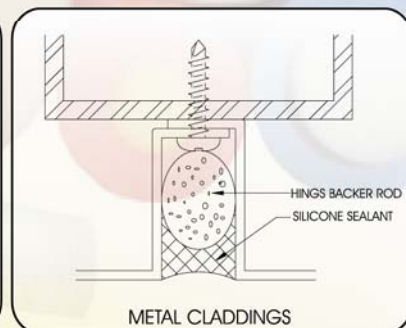
METAL CLADDINGS
